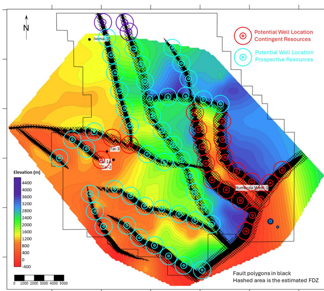
Figure 4.1: Top Basement depth map with potential well locations
