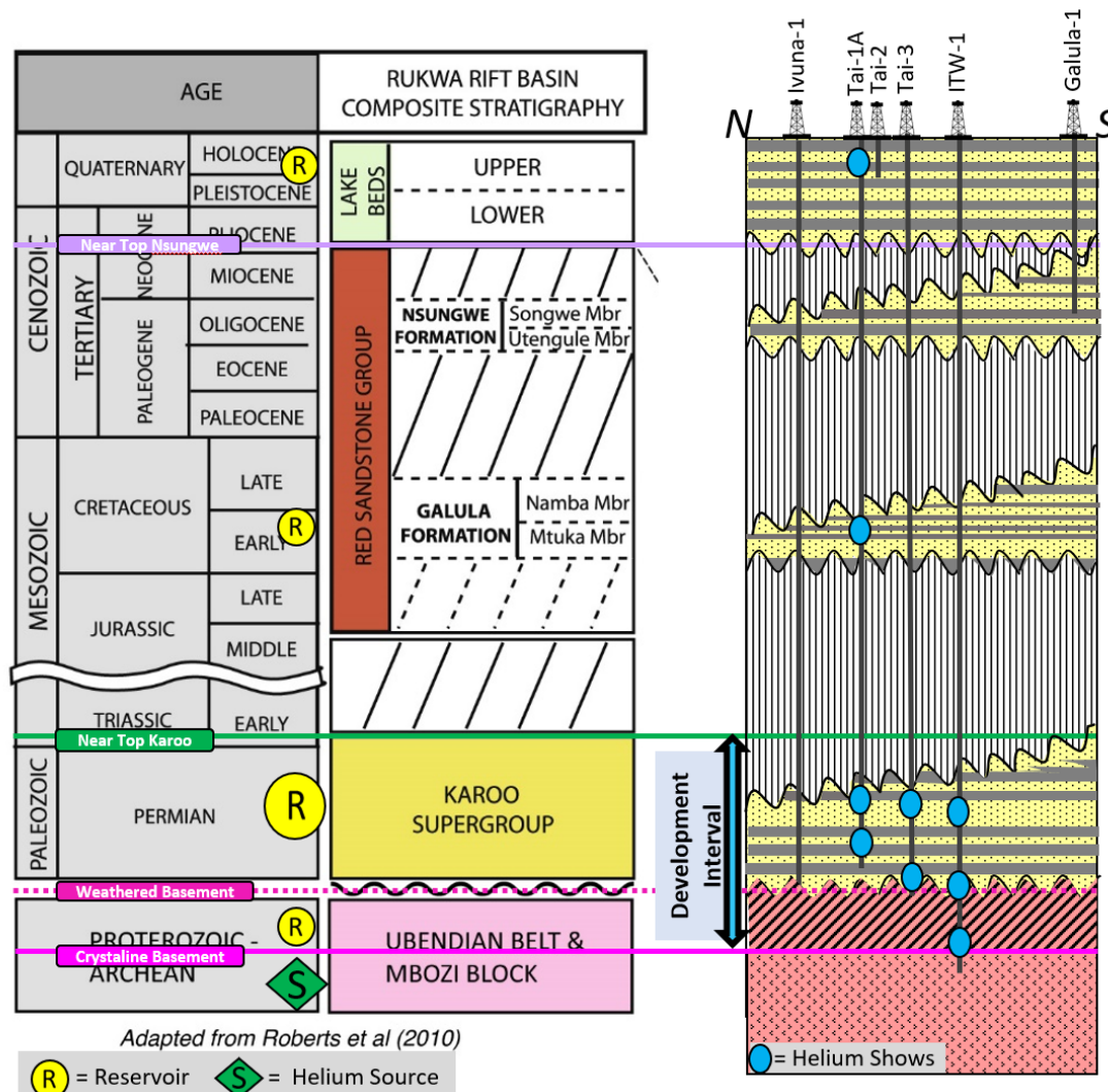
Figure 3.3: Regional Stratigraphic Column.
