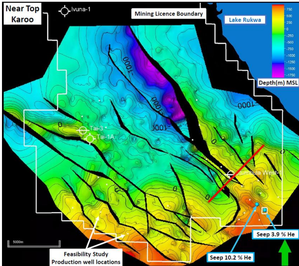
Figure 3.5: Top Karoo depth structure map
