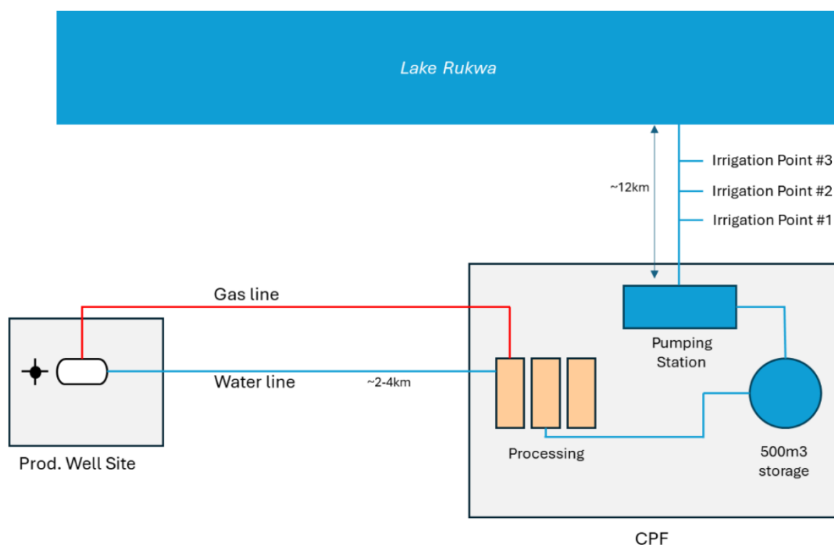
Figure 3.15: Schematic of production system layout (NB diagram shows only one wellsite, but there will be multiple)
