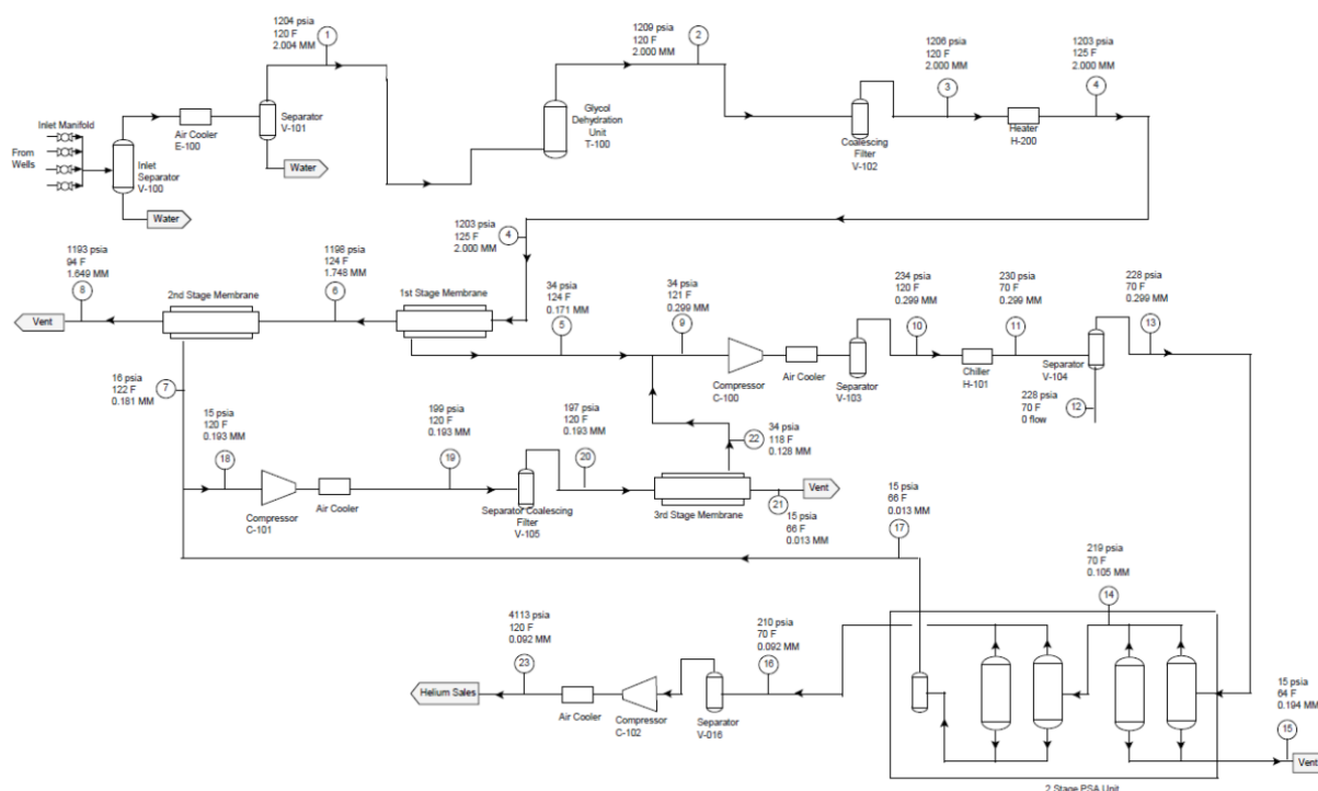
Figure 3.16: Process flowsheet for Central Production Facility (CPF)
