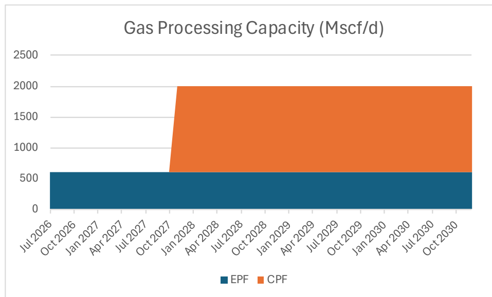
Figure 3.18 Gas Processing Capacity Schedule
