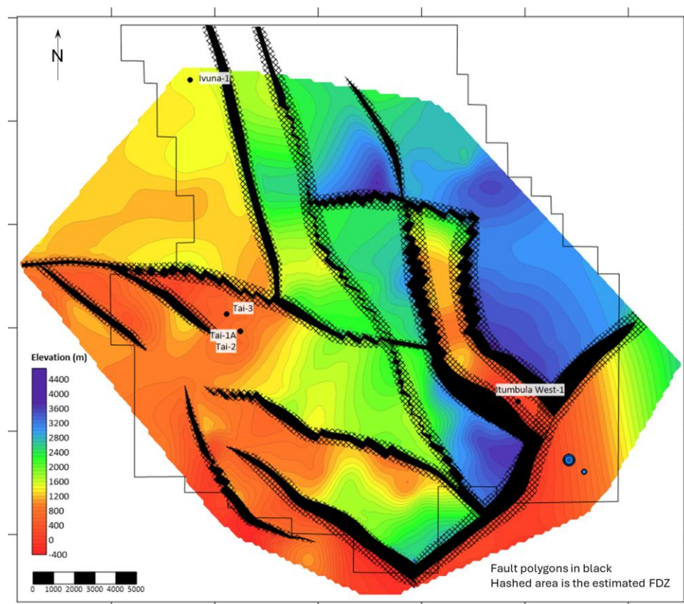
Figure 3.8: Top Basement depth structure map (based on Helium One) with Fault Damage Zones (FDZ).
