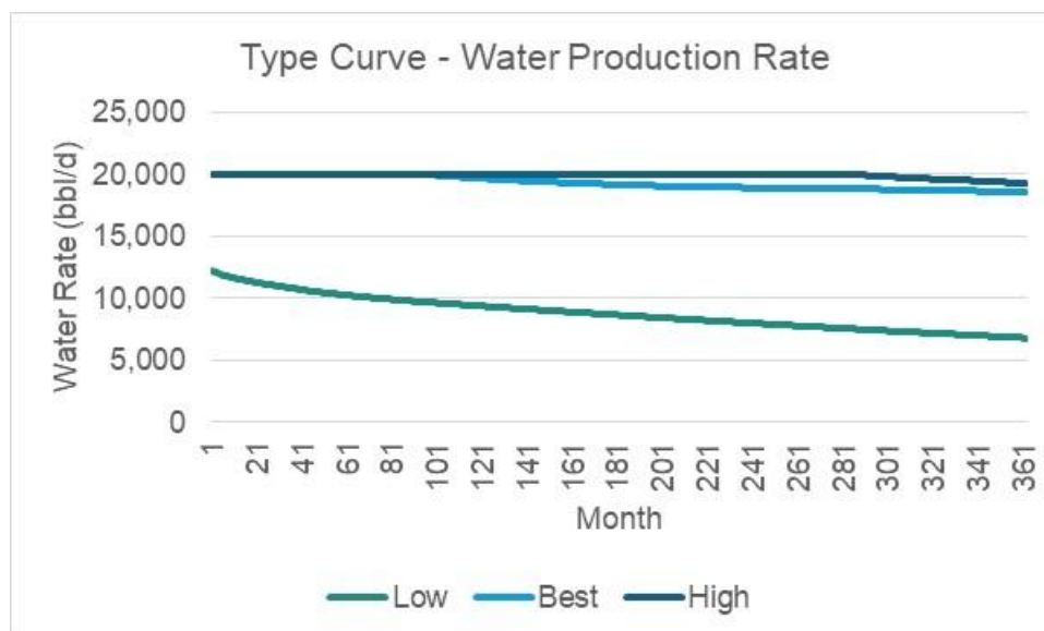
Figure 3.13: Low – best – high water production rate type curve
