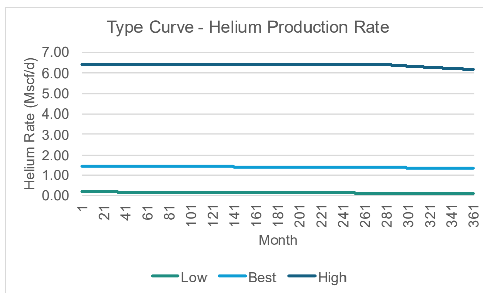
Figure 3.14: Low – best – high helium production rate type curve
