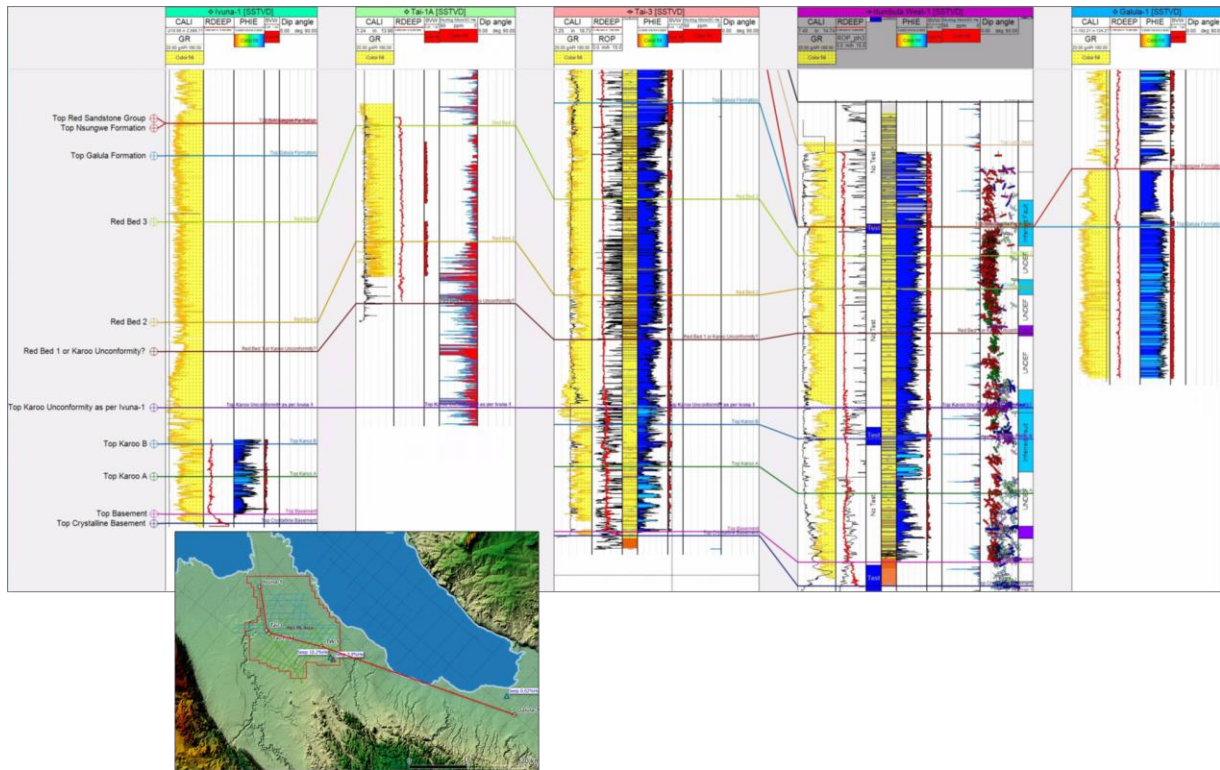
Figure 3.2: Well correlation panel
