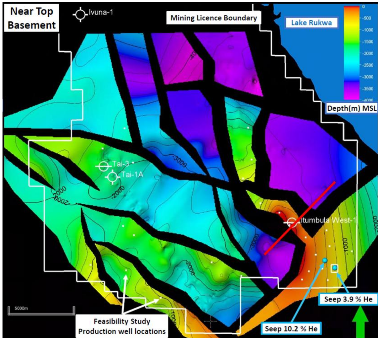
Figure 3.6: Top Basement depth structure map
