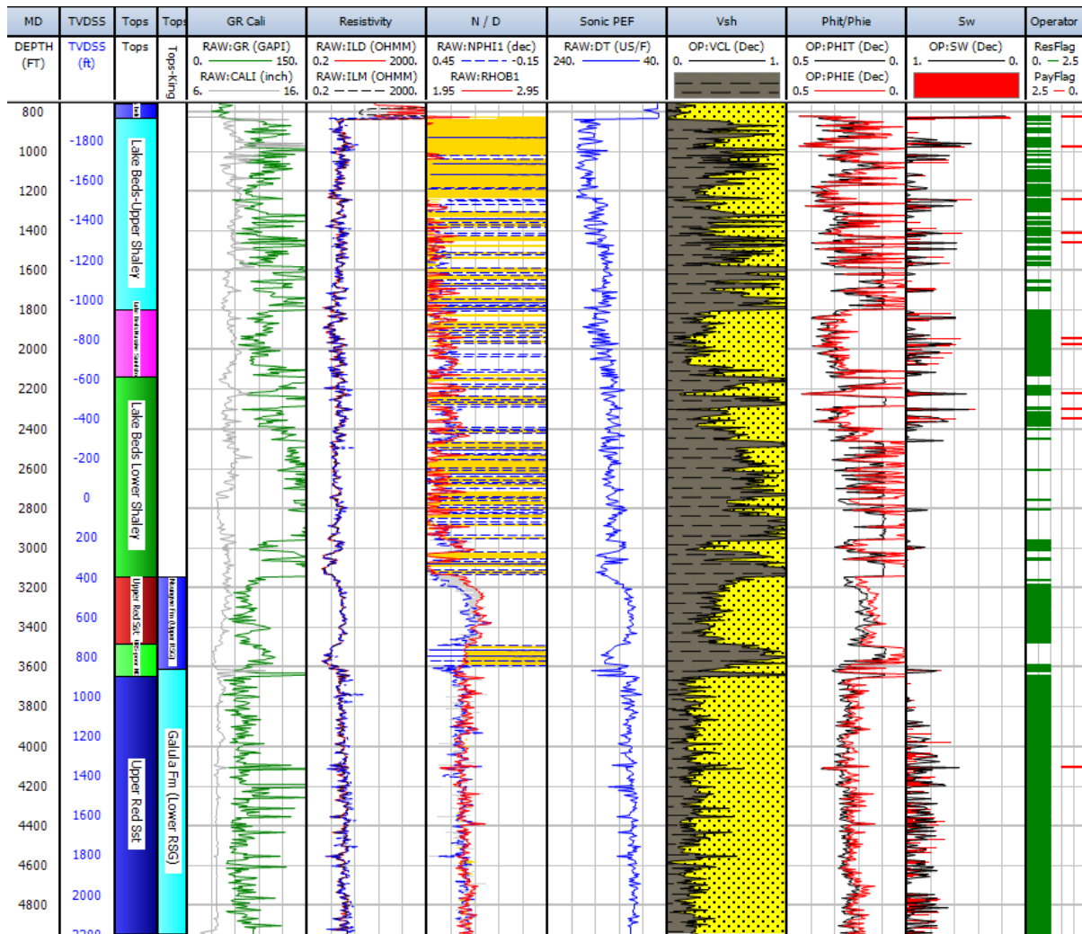
Figure 3.10: Well Galula-1 CPI
