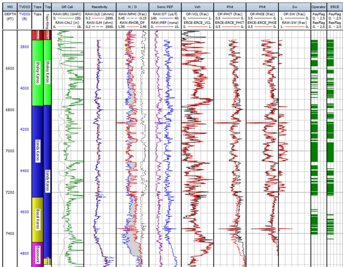
Figure 3.9 Well Ivuna-1 CPI (ERCE interpretation-red, Operator interpretation-black)
