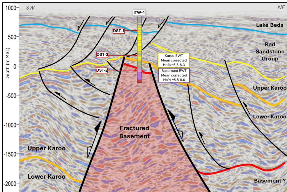
Figure 3.7: Interpreted seismic section through Itumbula-1 Well.
